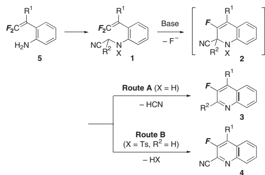
Scheme 1. Synthetic strategy for 3-fluoroquinolines.
